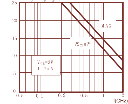
INSERTION POWER GAIN, MAG vs. FREQUENCY
