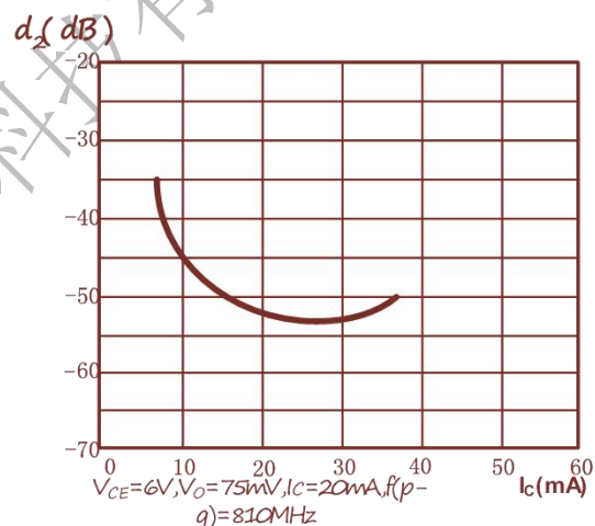
DISTORTION vs. FUNCTION of COLLECTOR CURRENT
