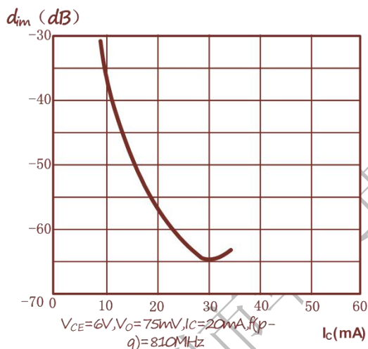
vs. FUNCTION of COLLECTOR CURRENT
