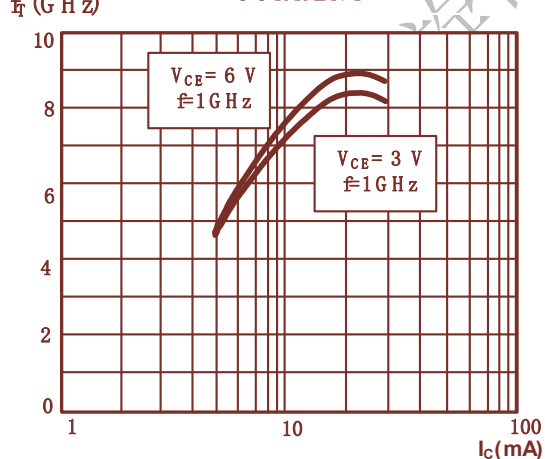
FREQUENCY vs. COLLECTOR CURRENT
