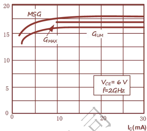
GAIN vs. FUNCTION of gain(GHz) COLLECTOR CURRENT
