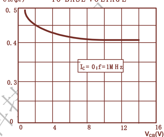
REVERSE TRANSFER CAPACITANCES. COLLECTOR TO BASE VOLTAGE
